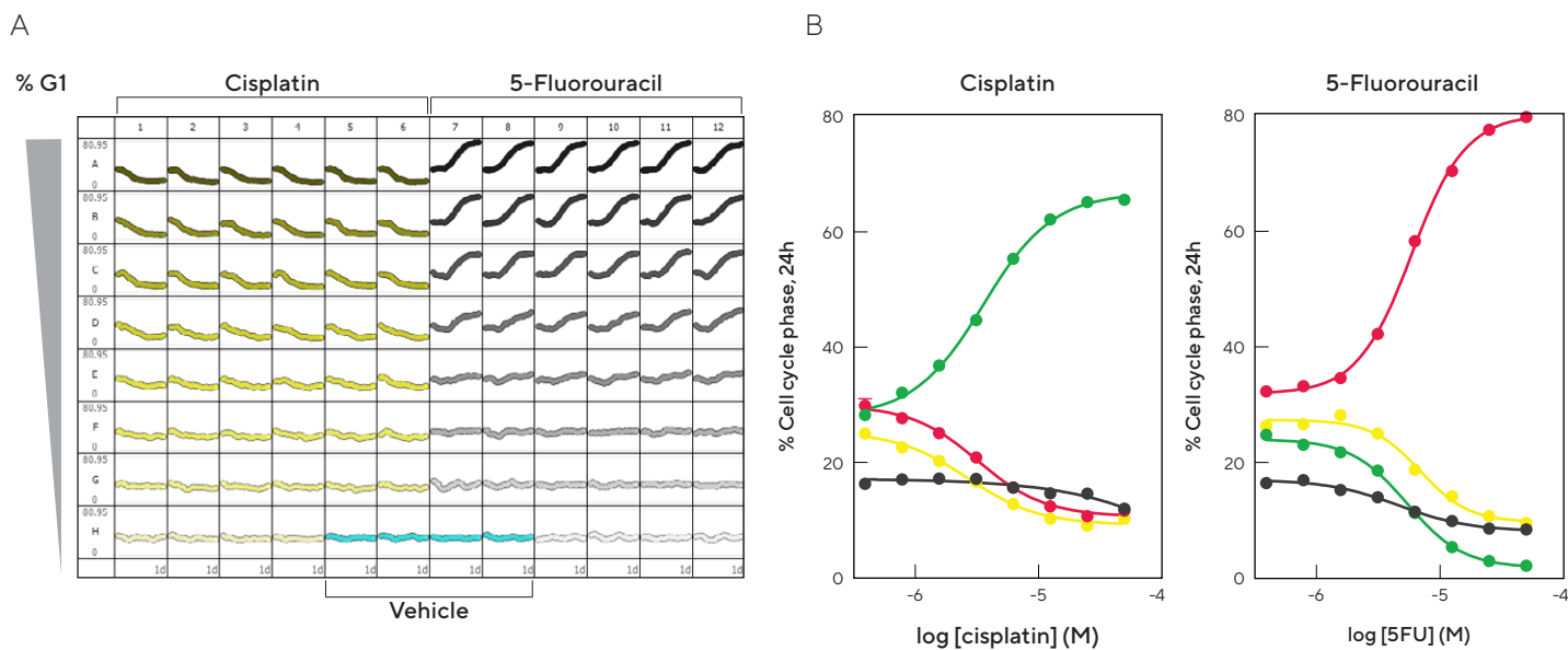
Figure 5: Concentration dependence of cell cycle modulators. HT1080 cells expressing Incucyte ® Cell Cycle were treated with cisplatin (0–50 \mu M) or 5-fluorouracil (5-FU, 0–50 \mu M). Plate view shows the time course of percentage of cells in G1 phase in each well of a 96-well plate, over 1 day treatment with cisplatin or 5-FU. A) Concentration response curves indicate the efficacy of cisplatin and 5-FU at 1 d and percent change in each population over the concentration ranges tested (B).
