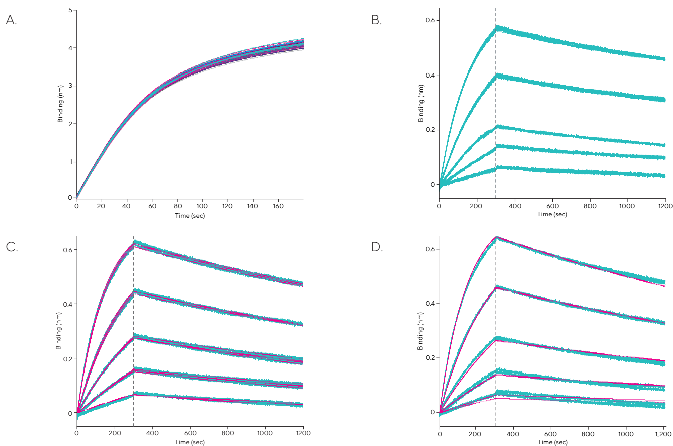
Figure 2: Octet ® comparability kinetics studies showing side by side kinetics data for biotinylated anti-PSA antibody immobilized on two different lots of SAX2 Biosensors binding to PSA antigen. (A) An overlay of the immobilization data from three instruments where PSA antigen was used at 200 nM, 100 nM, 50 nM, 25 nM and 12.5 nM using the Octet ® R8 (B), Octet ® RH16 (C) and Octet ® RH96 (D) systems. Data was acquired in duplicates for each biosensor lot. Only one lot was used on the Octet ® HTX system. Experiments were run at 25°C using the 8-channel read head mode for all three Octet ® models.
