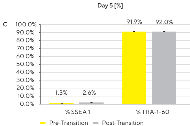
Figure 2. hPSC cultures transitioned from mTeSR1 to NutriStem® hPSC Medium exhibit similar levels of pluripotency marker expression. Pluripotency was measured both pre- and post-transition from mTeSR1 to NutriStem® hPSC Medium (with additional 100ng/mL bFGF added). Prior to the transition, active hPSC cultures in mTeSR1 were assessed via immunocytochemistry for the nuclear pluripotency marker Nanog (Fig. 2, A) as well as by flow cytometry for SSEA1 and TRA-1-60 (Fig. 2, C). Following transition of hPSCs to NutriStem® hPSC Medium, cultures were also assessed via immunocytochemistry for the nuclear pluripotency marker Nanog (Fig. 2, B) as well as by flow cytometry for SSEA1 and TRA-1-60 (Fig. 2, C) demonstrating that hPSC cultures transitioned into NutriStem® hPSC Medium result in similarly high levels of pluripotency (Fig. 2, C) when compared to hPSC cultures maintained in mTeSR1.
